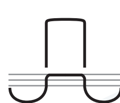
Outward Clinch
